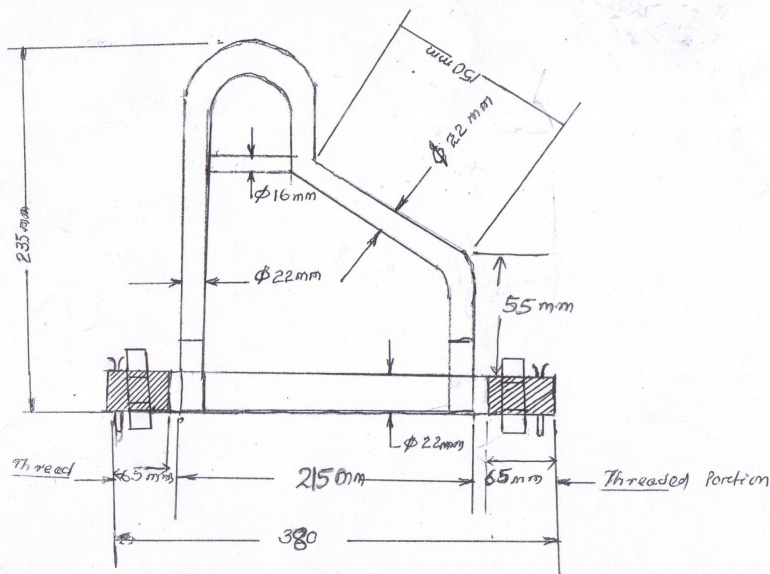
HANGER FOR 132 KV PA TYPE TOWER
